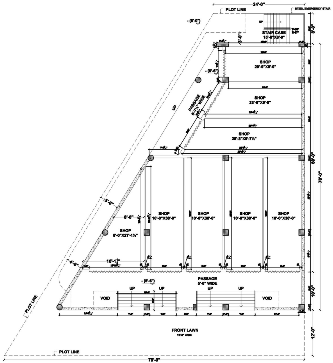
BASEMENT FLOOR PLAN SCALE: 1"=8'-0"
